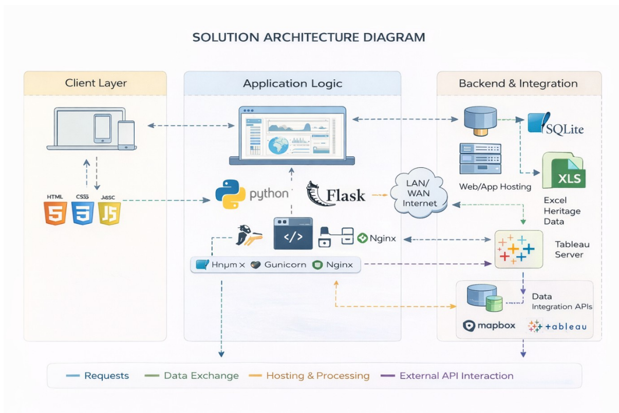
Figure 1: Solution Architecture
